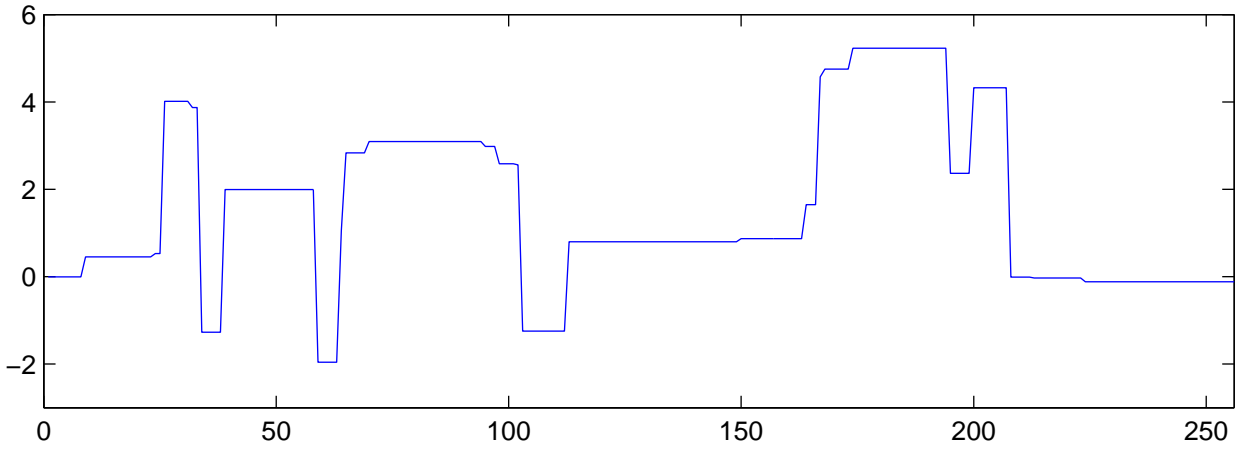
Moreau-enhanced Total Variation Denoising (gamma = 0.7)
