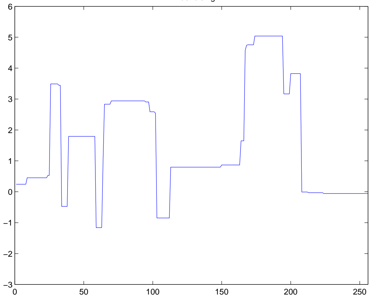
TV denoising
