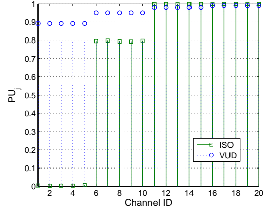
Fig. 5. ISO vs. VUD: heterogeneous streaming rates among channels. There are 4 streaming rates: channels 1-5 with 2r ; channels 5-10 with 1.5r ; channel 11-15 with r ; channels 16-20 with 0.5r . VUD also achieves higher PU_j for high-rate channels.
